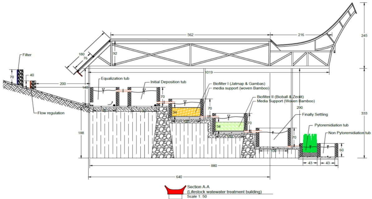
Fig. 2 Waste treatment building
