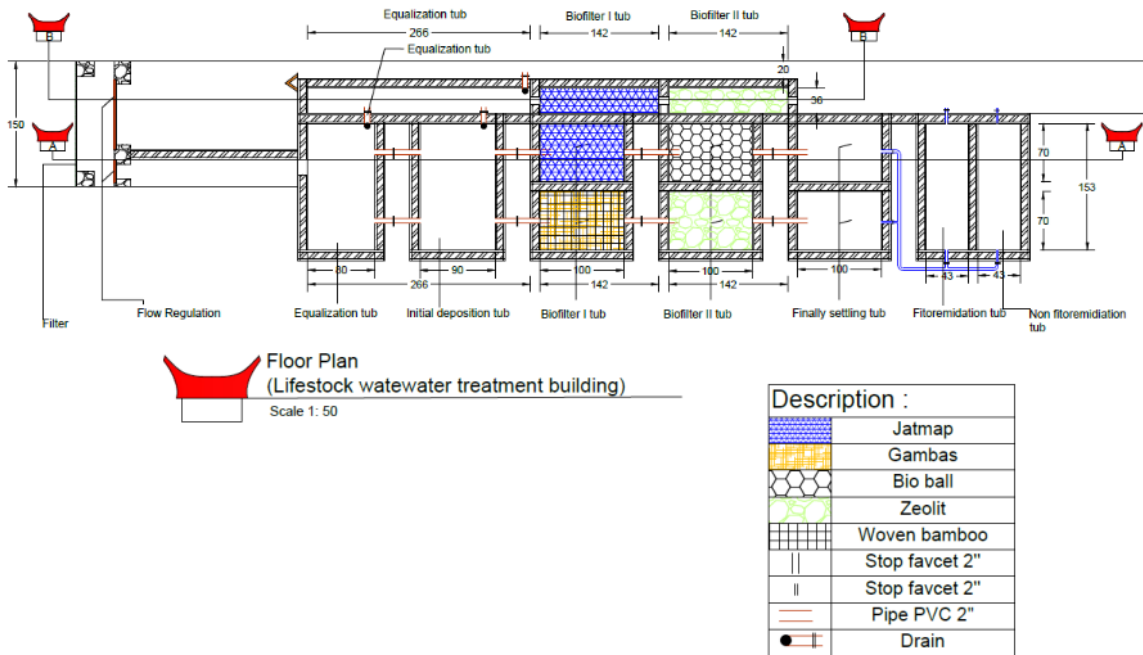
Fig. 4 Waste Treatment Building
